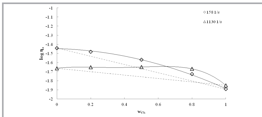
Figure 3. Logarithm of apparent shear viscosity of Ch and HPAM and their blends versus weight fraction of Ch in the blend; T = 298\text{ K} , solvent: 0.1\text{M CH}_3\text{COOH}/0.2\text{NaCl} , dotted line - the values calculated according to the additivity rule.
