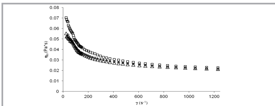
Figure 2. Apparent shear viscosity versus shear rate of 1% HPAM solution, T = 298 \text{ K} , solvent: \square - water, \diamond - 0.1 M \text{CH}_3\text{COOH}/0.2 \text{ NaCl} , \Delta - 0.1 M \text{CH}_3\text{COOH} .
