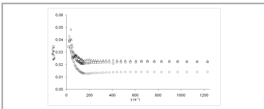
Figure 1. Apparent shear viscosity versus shear rate of 1% chitosan solution, T = 298\text{K} , solvent: \square - 0.1 M \text{CH}_3\text{COOH} , \diamond - 0.1 M \text{CH}_3\text{COOH}/0.2 \text{ NaCl} , \Delta - 0.1 M \text{CH}_3\text{CH}(\text{OH})\text{COOH} .
