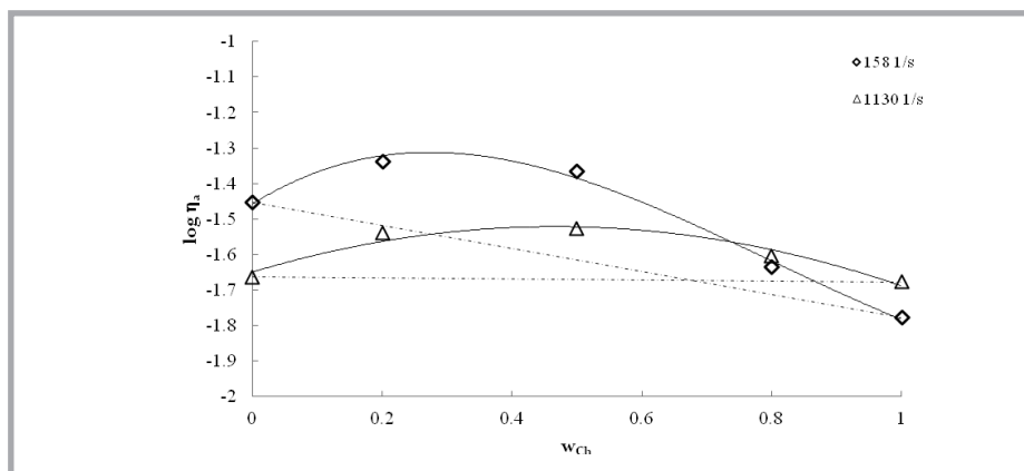
Figure 4. Logarithm of apparent shear viscosity of Ch and HPAM and their blends versus weight fraction of Ch in the blend; T = 298\text{ K} , solvent: 0.1\text{ M CH}_3\text{COOH} , dotted line - the values calculated according to the additivity rule.
